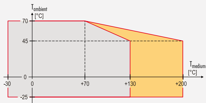
Temperature diagram
